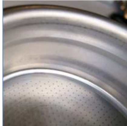
NEW FILTER BASKET (F.3.028.01)
