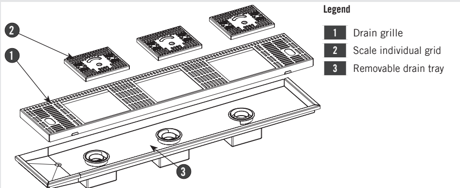
Fig. 3 - Precision scale - 2, 3 and 4 brewing groups
