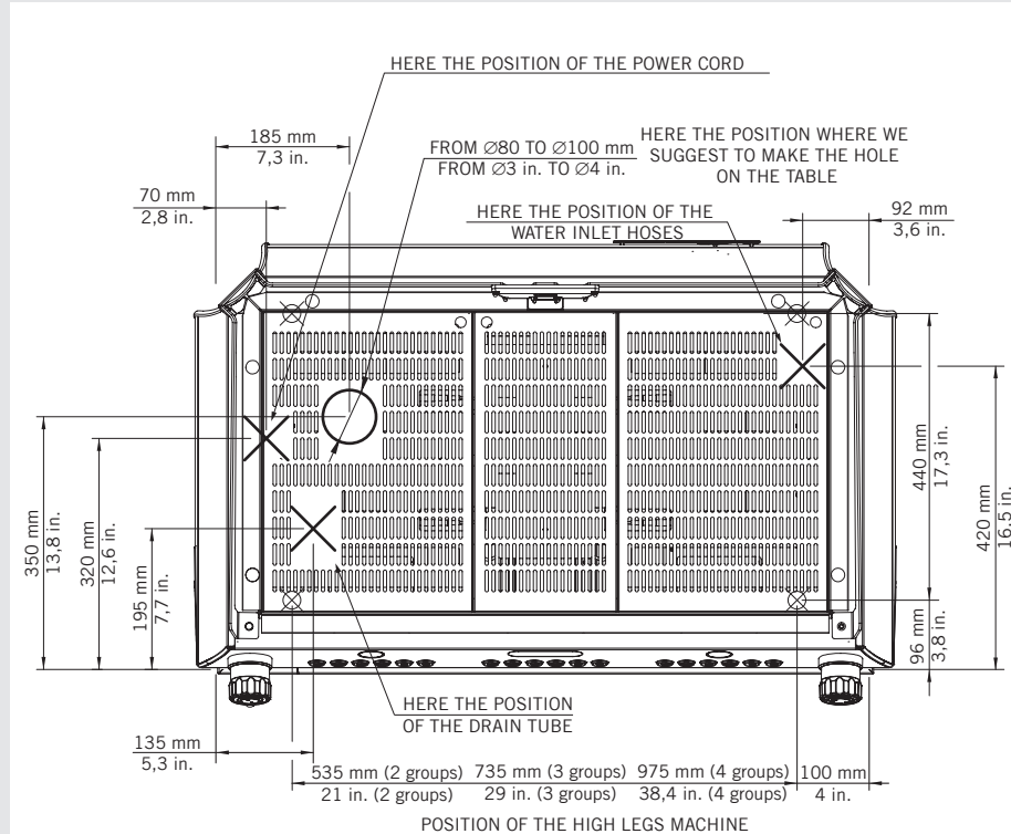
Fig. 2 - Installation guide
